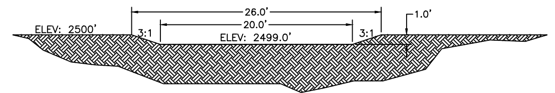
SUMP EMERGENCY SPILLWAY SECTION SCALE: 1"=10'
