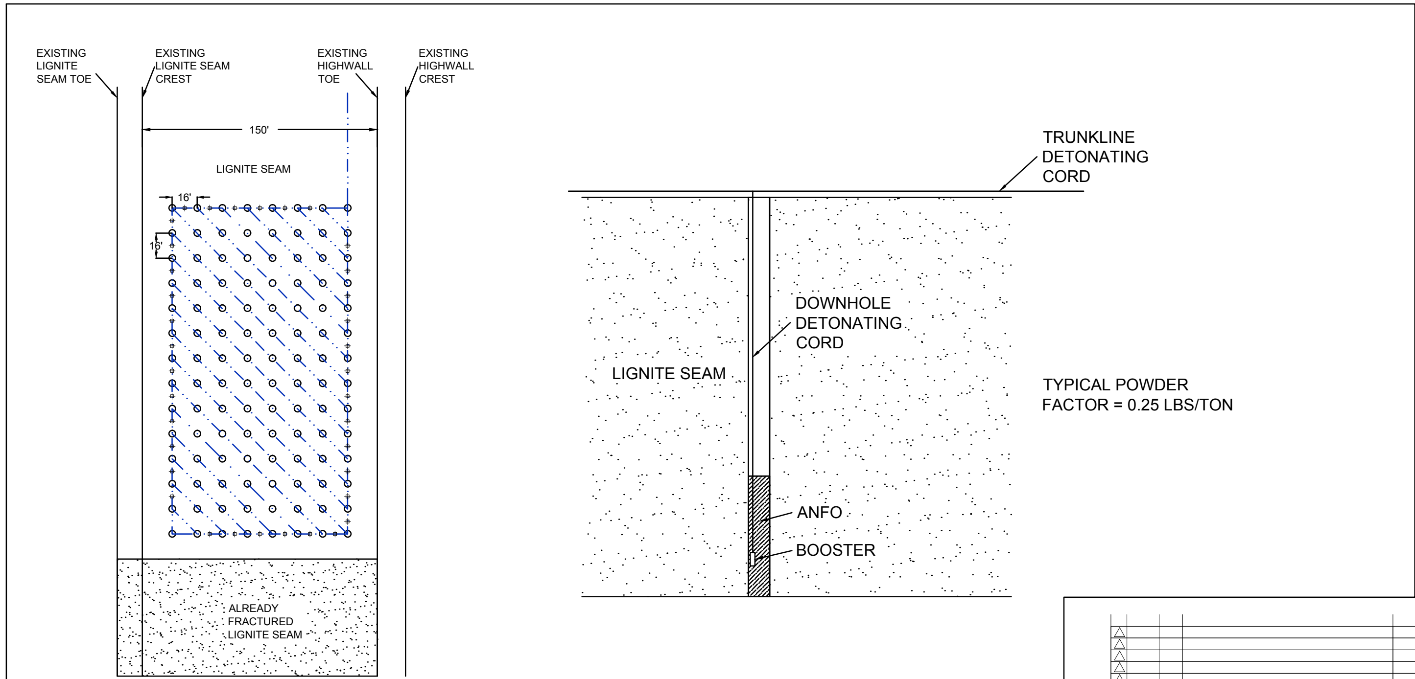
BLAST DESIGN PLAN VIEW
