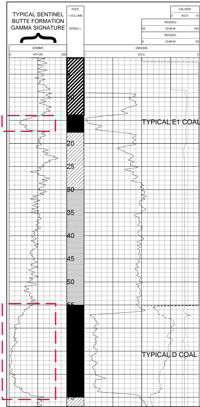
TYPICAL LOG
